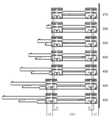
Cabinet track installation dimensions
