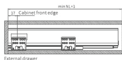
Slide rail installation dimensions
