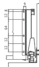
Back-panel mounting size
