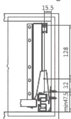
Front Connector panel mounting size
