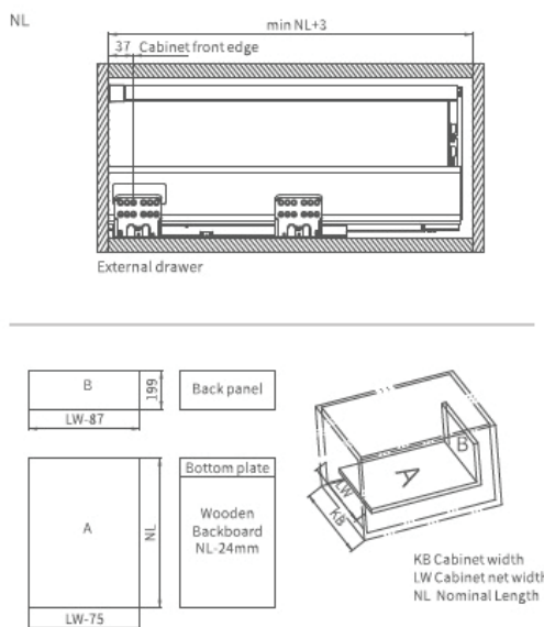
Slide mounting size
