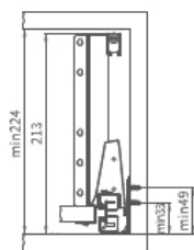
Space requirements of the inner cabinet installation
