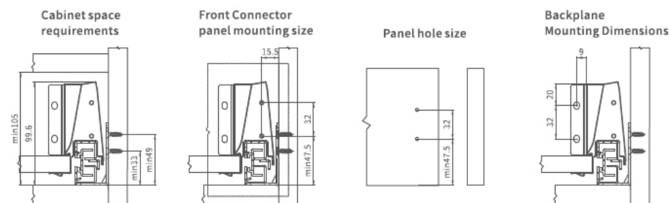
Cabinet track installation dimensions
