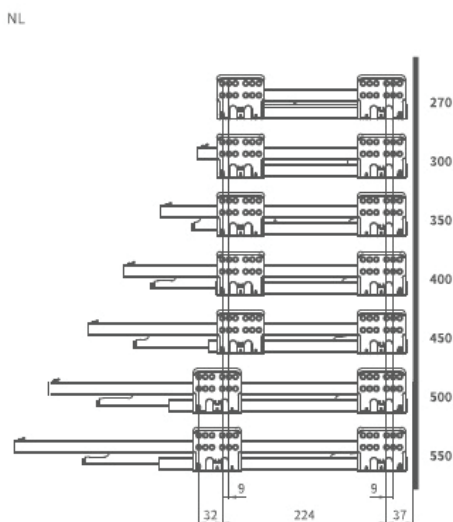
Cabinet slide mounting size
